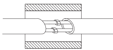
Thermal insulation
